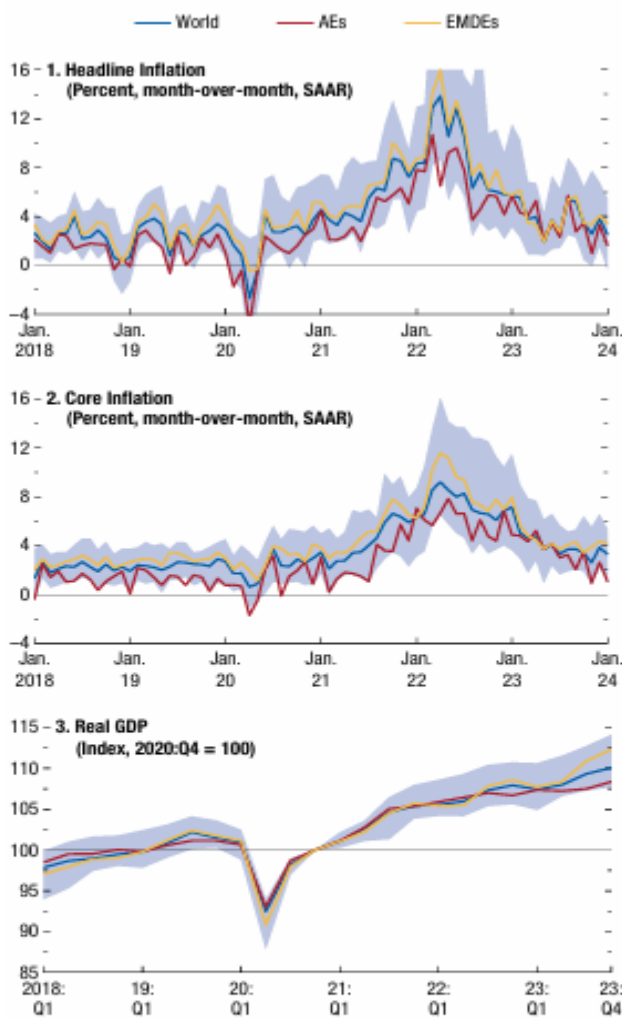
Figure 1.1. Global Inflation Falling as Output Grows
