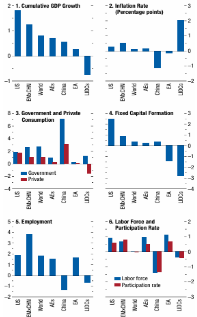
Figure 1.2. Performance in 2022–23 Compared with Projections at Time of Cost-of-Living Crisis
