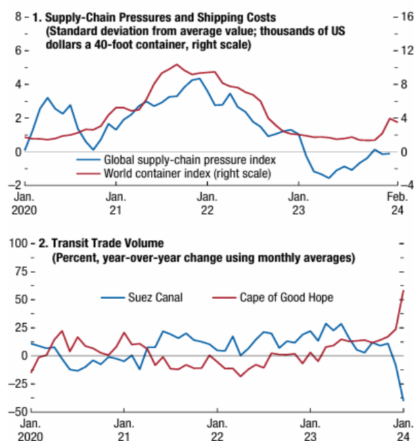
Figure 1.4. Supply-Chain Pressures and Red Sea Tensions
